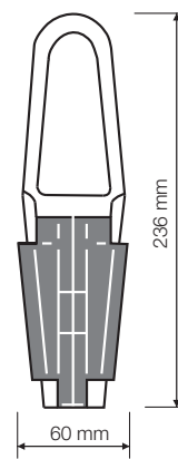
Mounting bracket for MJK Expert™ 7060 level transmitter
