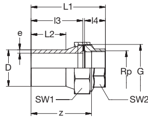
25.54.02.103 PE100-V2A Ü-Verschraubung lang IG-zyl Flachdichtring-EPDM SDR11 schwarz PE100-Stainless steel Transition-Union long female-thread-cyl flat-gasket-EPDM SDR11 black
